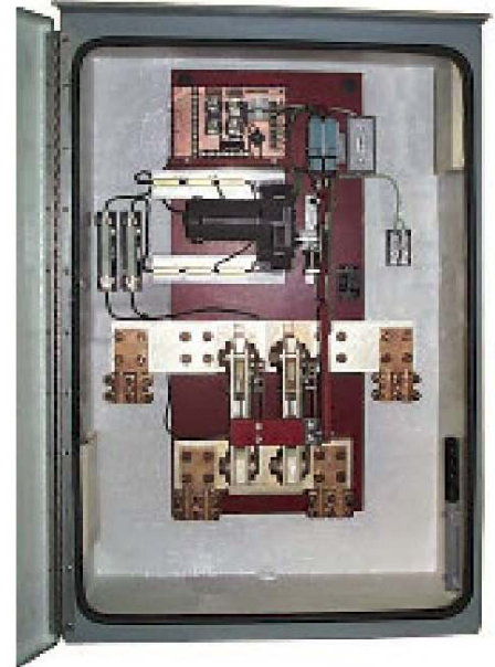
4000 AMP 1000 VDC MOTOR OPERATED TRACTION POWER DISCONNECT FOR STANCHION OR WALL MOUNTING
